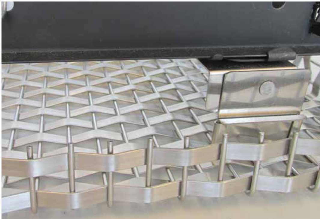
Atlantic fabric with clip attachment and T grid mounting
